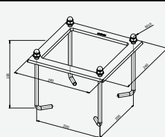
Art. 113 Anchoring support Namsos
