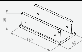
Art. 1906 Reinforced galvanized metal foot for Molde
